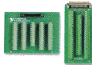
Figure 6. CB-68LP and CB-68LPR I/O Connector Blocks
