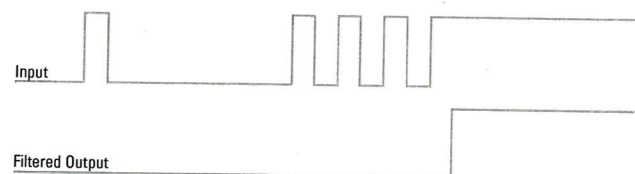
Figure 2. Debouncing and Glitch Removal
