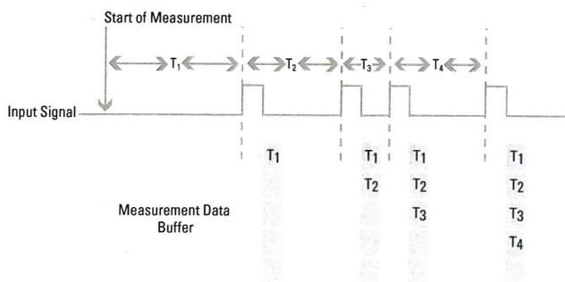
Figure 1. Buffered Period Measurement with Counter/Timers
