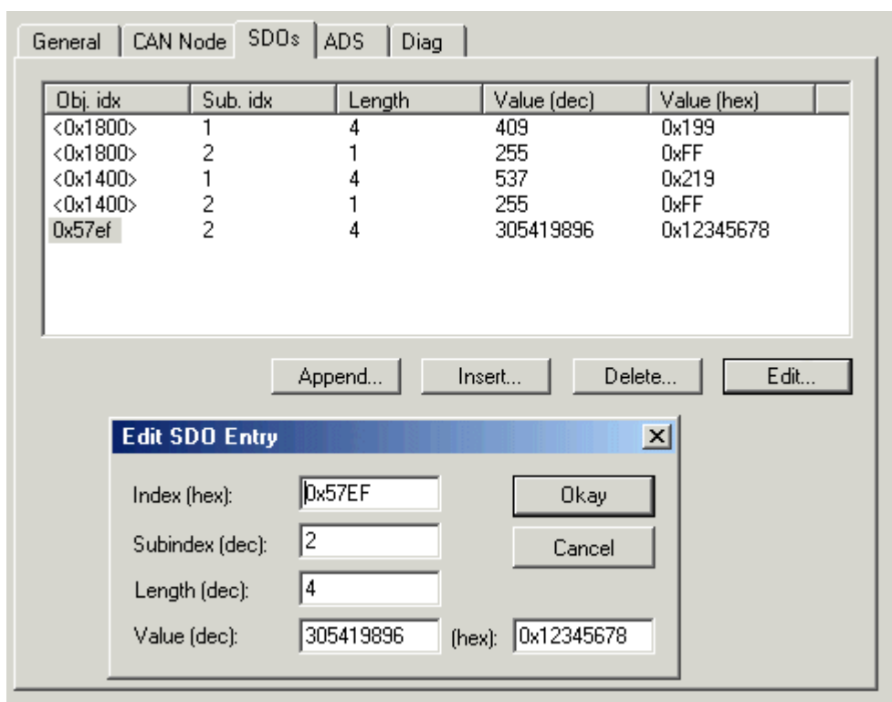
Fig. 122: SDO tab, editing an SDO entry
