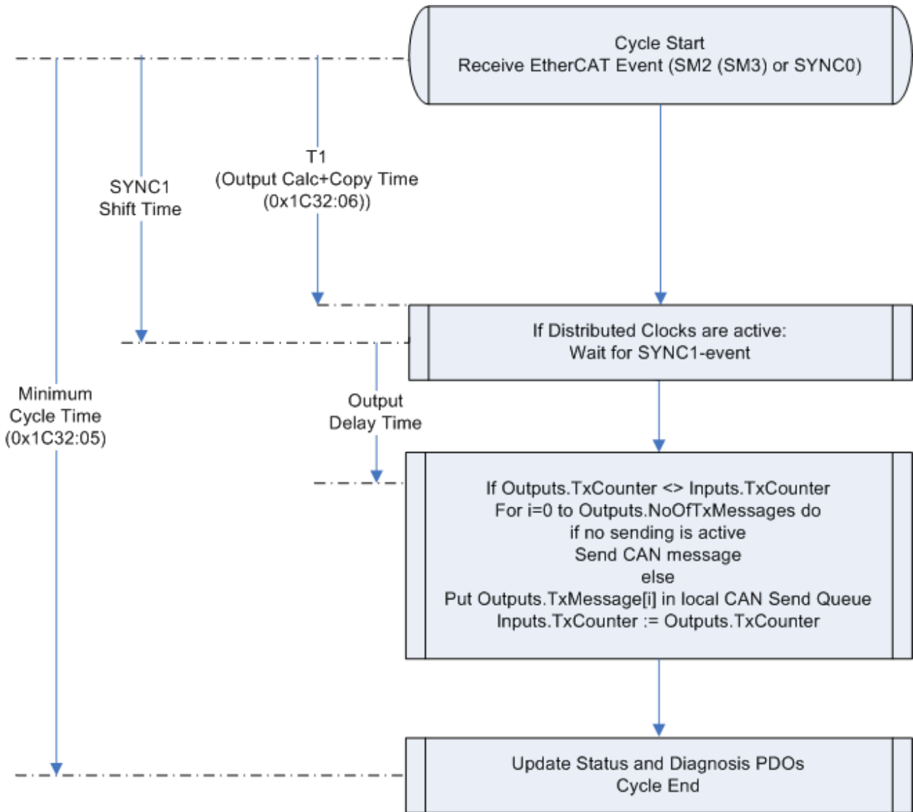
Fig. 133: Flow chart for CAN cycle in Fast CAN Queue mode
