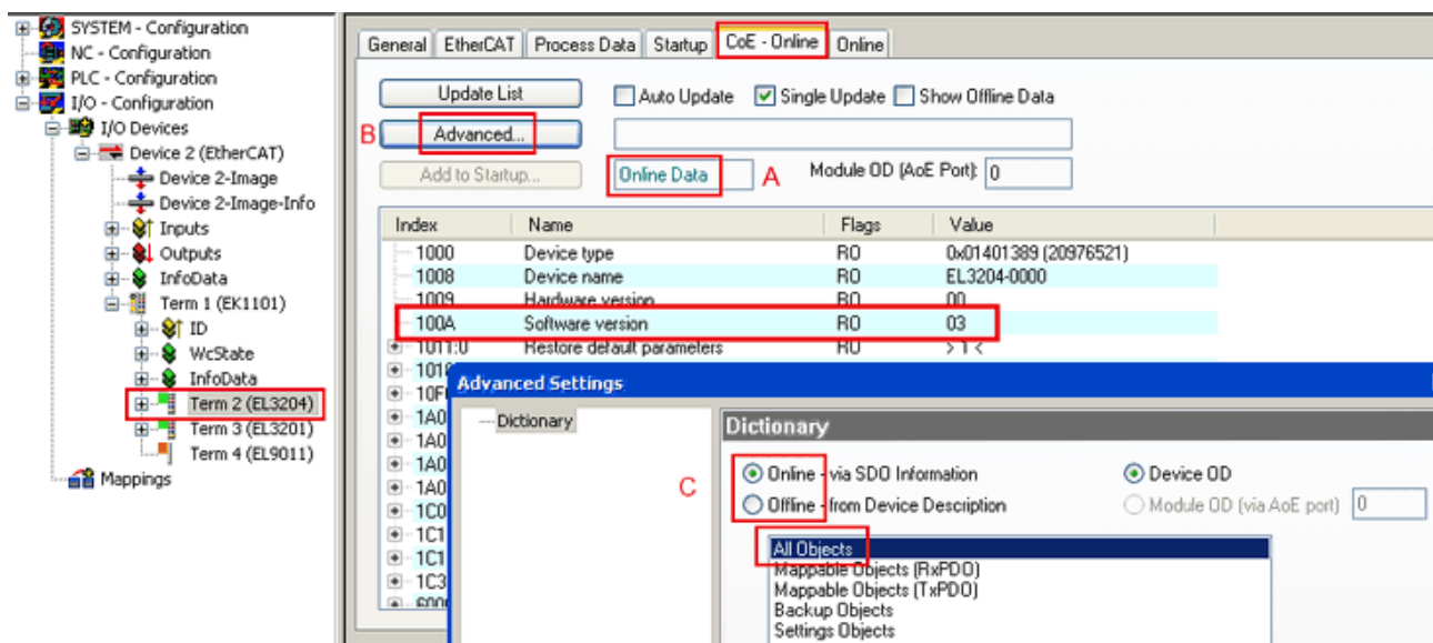
Fig. 146: Display of EL3204 firmware version
