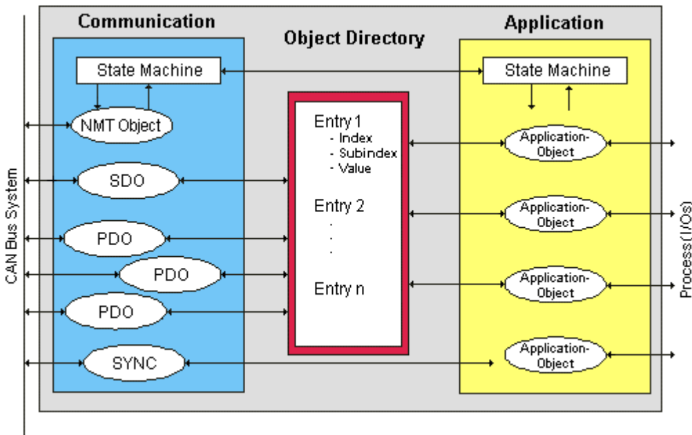
Fig. 13: CANopen Device Model
