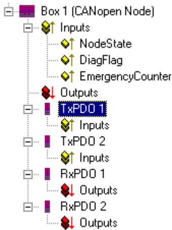
Fig. 108: TwinCAT tree: CANopen Box
