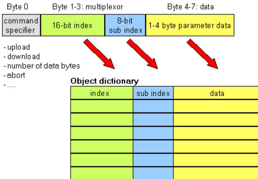
Fig. 121: SDO protocol: access to the object directory
