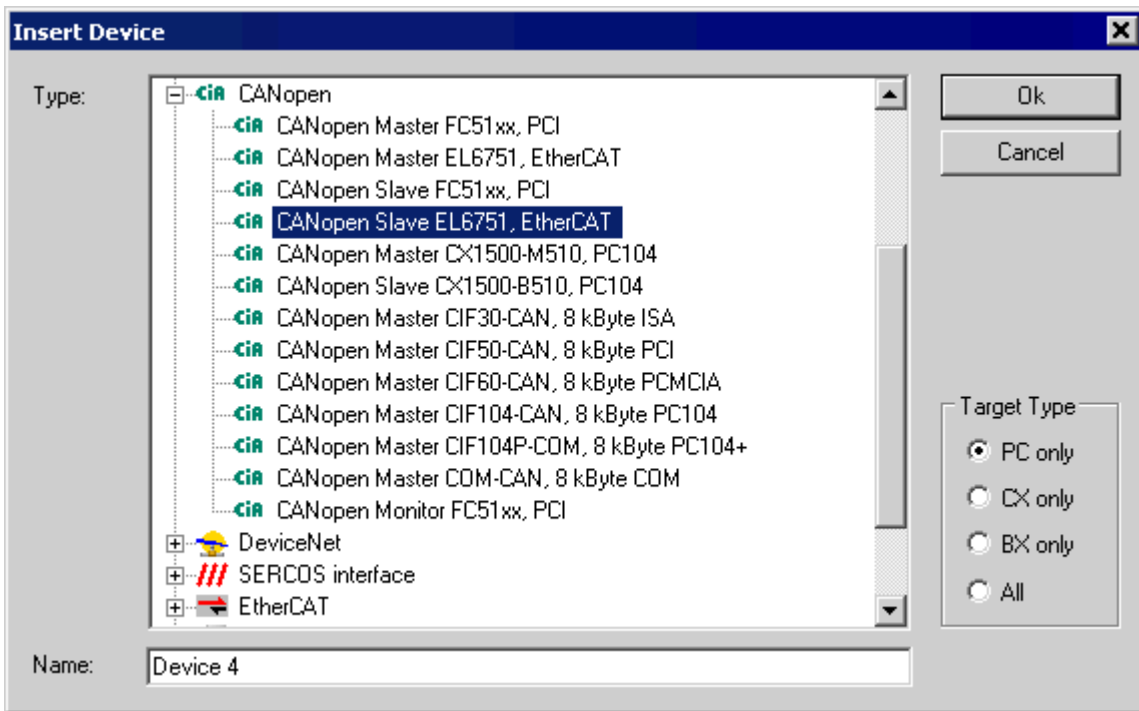
Fig. 98: EL6751-0010: Dialog "Appending an I/O device"
