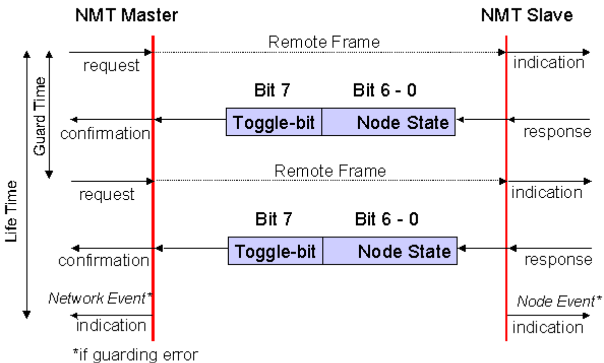
Fig. 112: Schematic diagram: "Guarding procedure"
