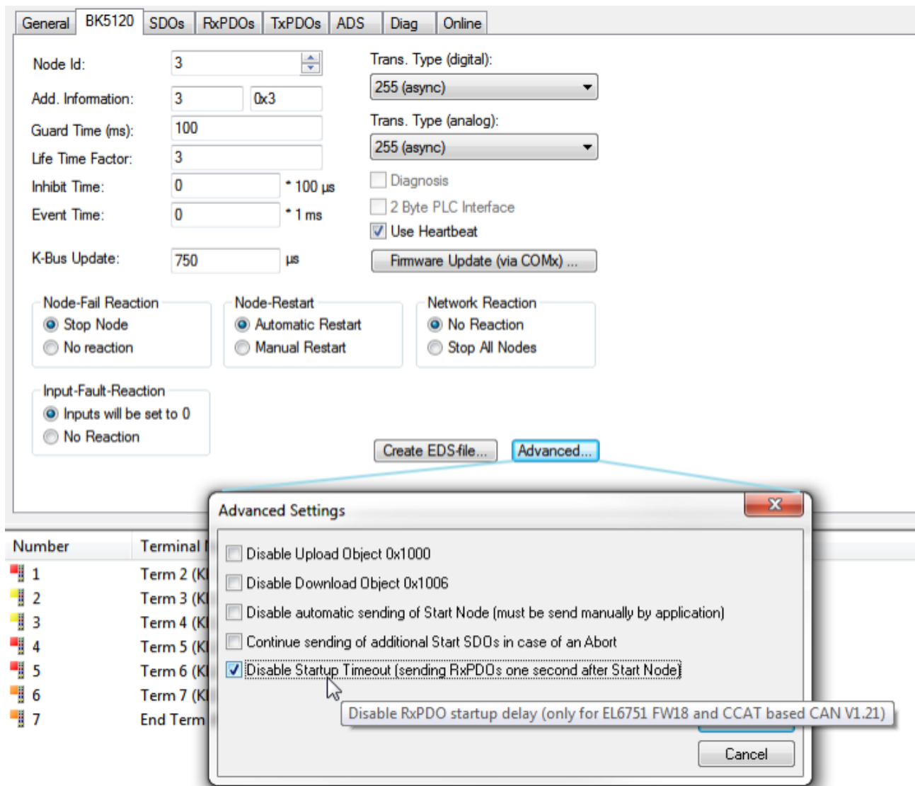
Fig. 125: Advanced Settings tab
