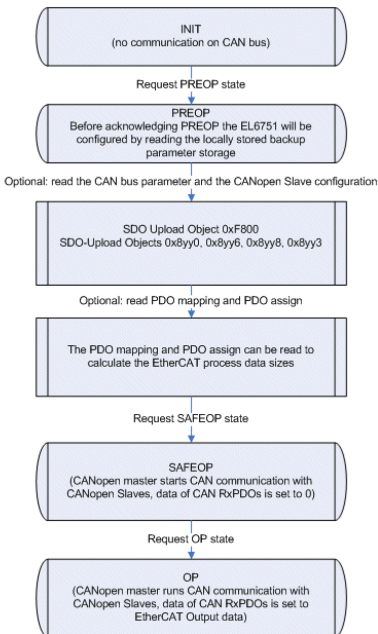
Fig. 128: Flow chart for EL6751 with Backup Parameter Storage
