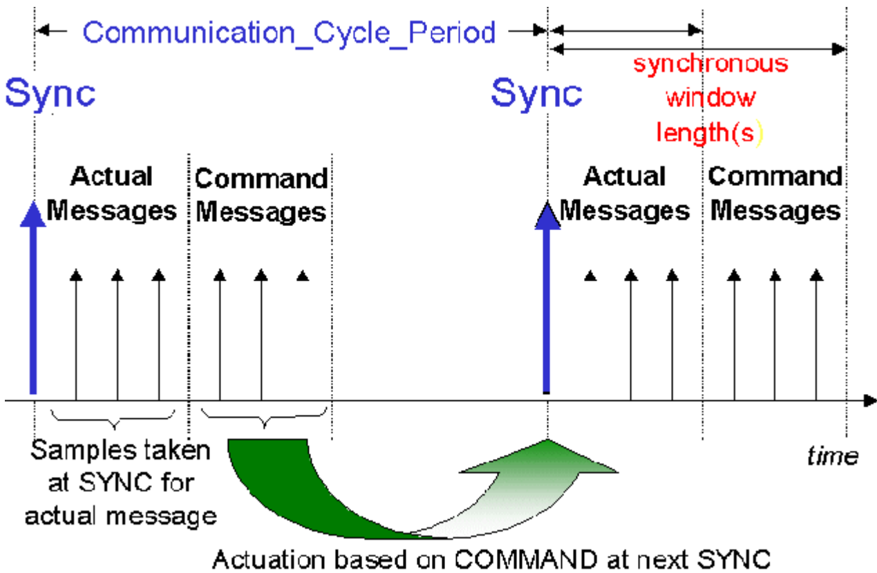
Fig. 117: Diagram: CAN "SYNC" telegram
