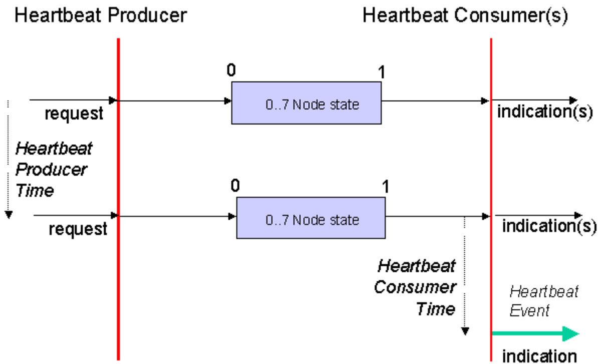
Fig. 113: Schematic diagram: "Heartbeat procedure"
