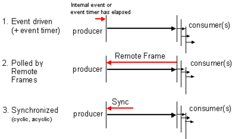
Fig. 116: Diagram: CAN process data transmission
