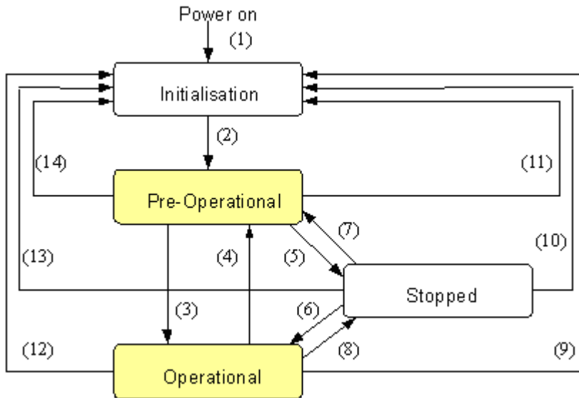
Fig. 111: CANopen bootup state diagram
