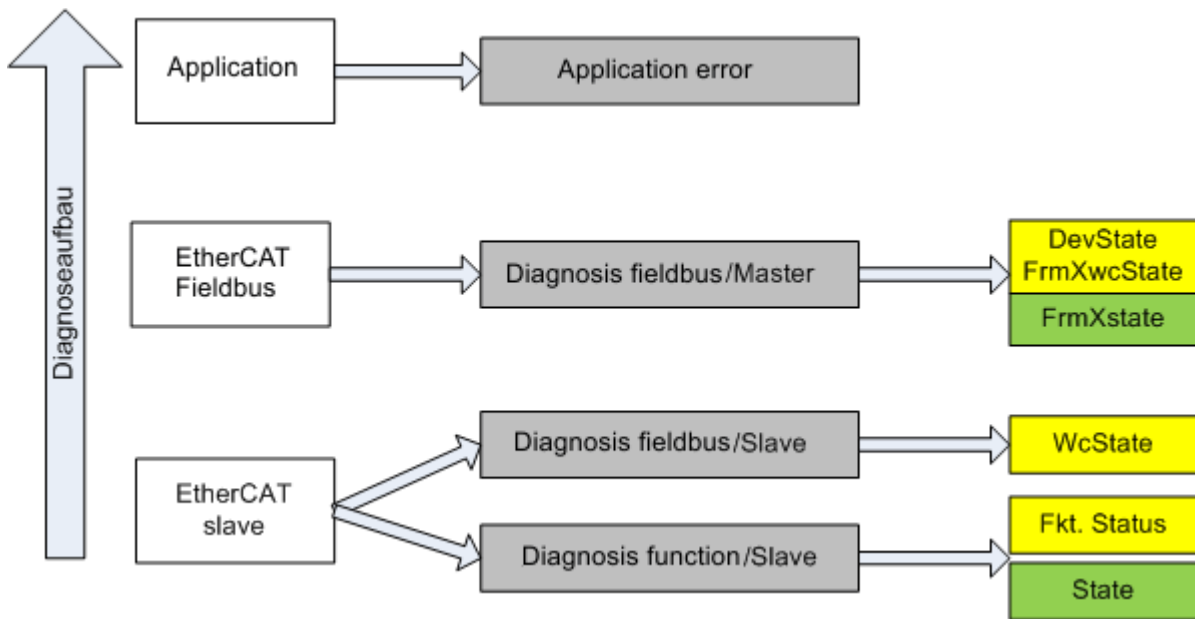
Fig. 80: Selection of the diagnostic information of an EtherCAT Slave
