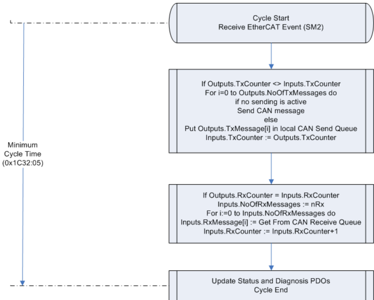
Fig. 132: Flow chart for CAN cycle in buffered CAN Queue mode
