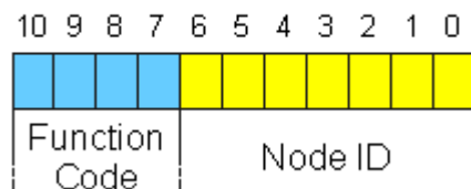
Fig. 124: Schematic: CANopen default identifier
