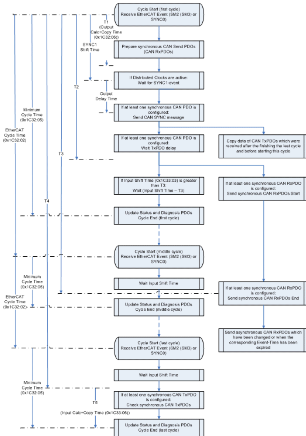
Fig. 130: Flow chart for CAN cycle (Sync Multiplier > 1)
