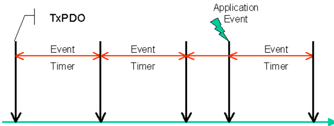
Fig. 119: Time representation of the event timer
