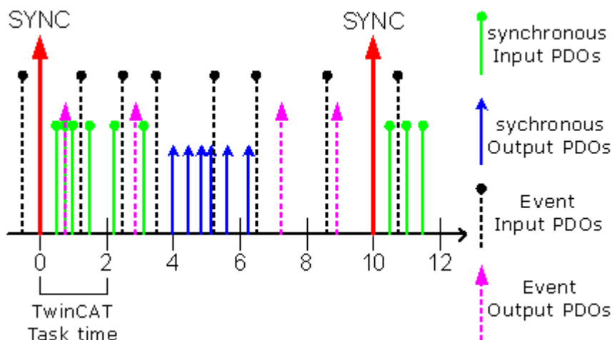
Fig. 92: Diagram: Sync-Tx-PDO-Delay sample
