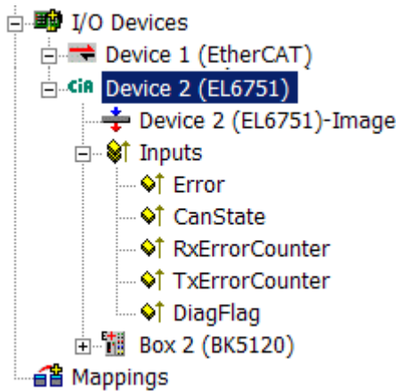
Fig. 137: TwinCAT tree: Diagnostic variables of the EL6751
