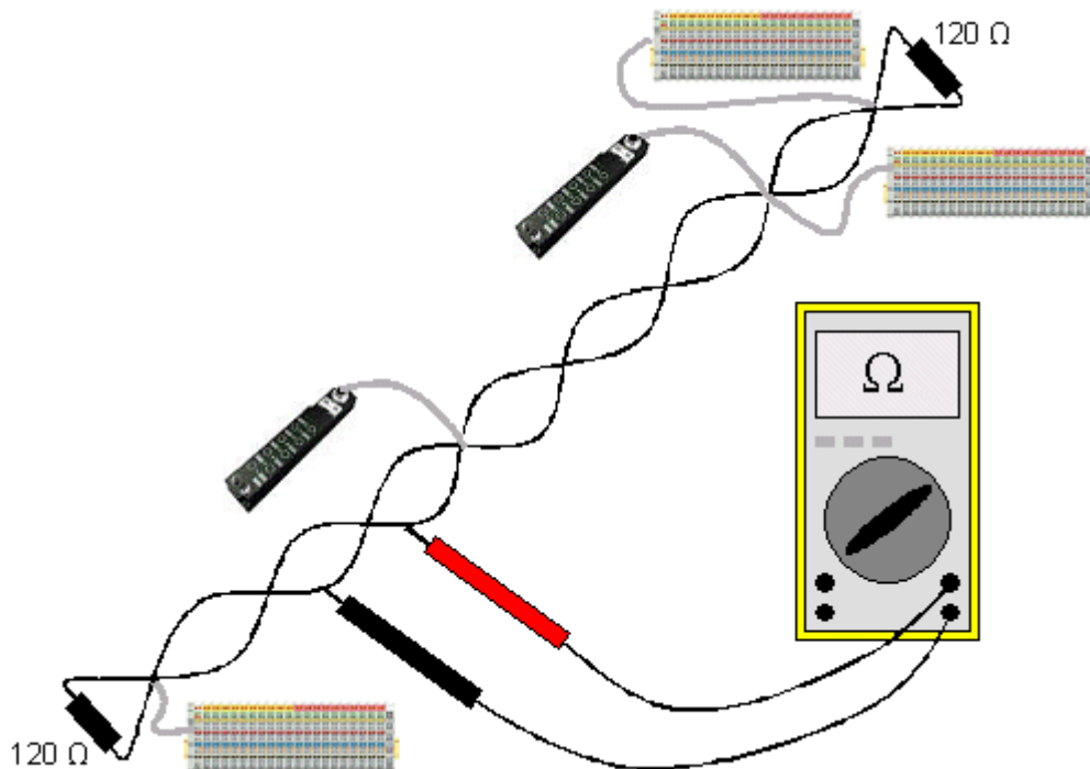
Fig. 139: Wiring diagram for test setup
