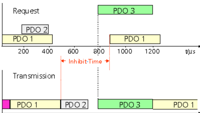
Fig. 118: Timing diagram: "Inhibit time"
