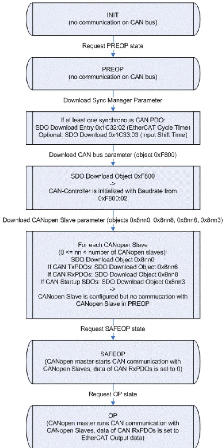
Fig. 126: Flow chart for the EL6751 with Start SDOs
