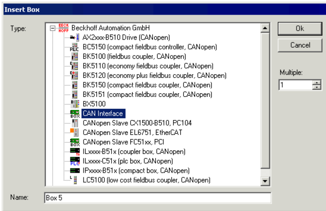
Fig. 94: Selection dialog "Inserting a box"
