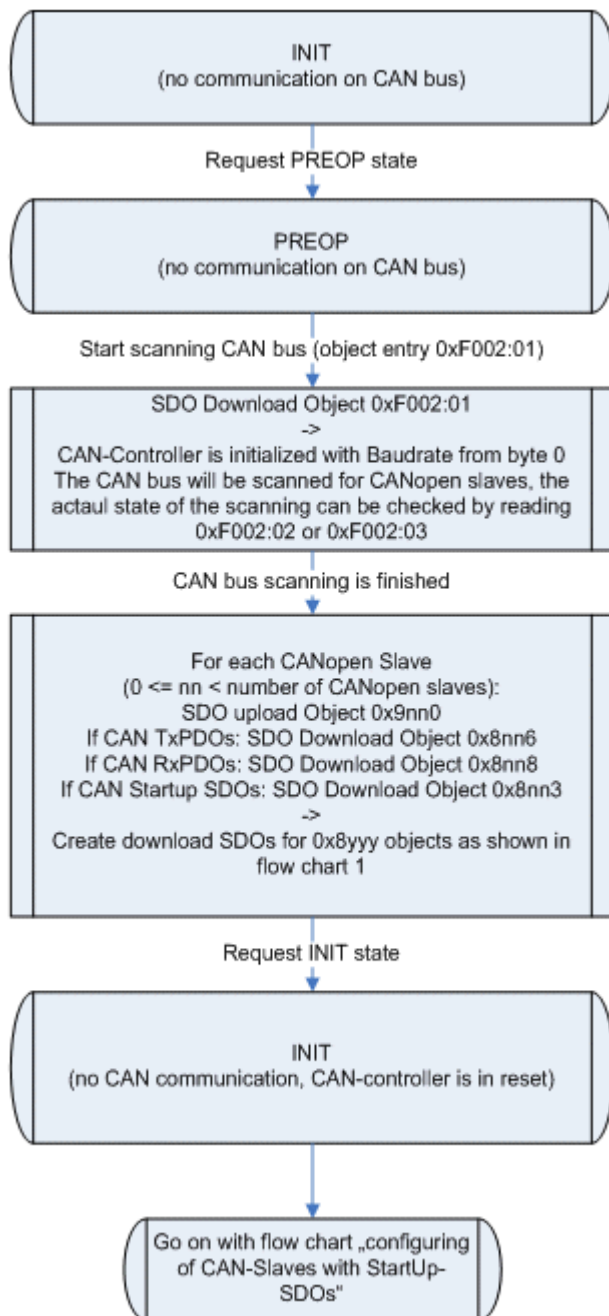
Fig. 127: Flow chart for EL6751 with scanning of the CAN bus
