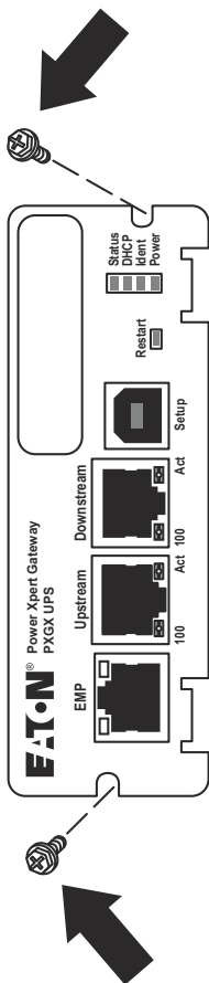
Figure 2. Secure the PXGX UPS Card
